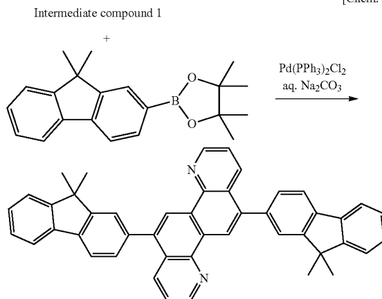
Example compound 1-1
