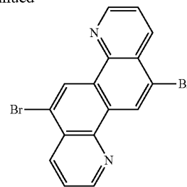
Intermediate compound 1
