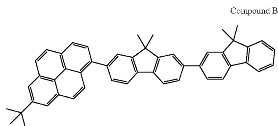
Compound B
